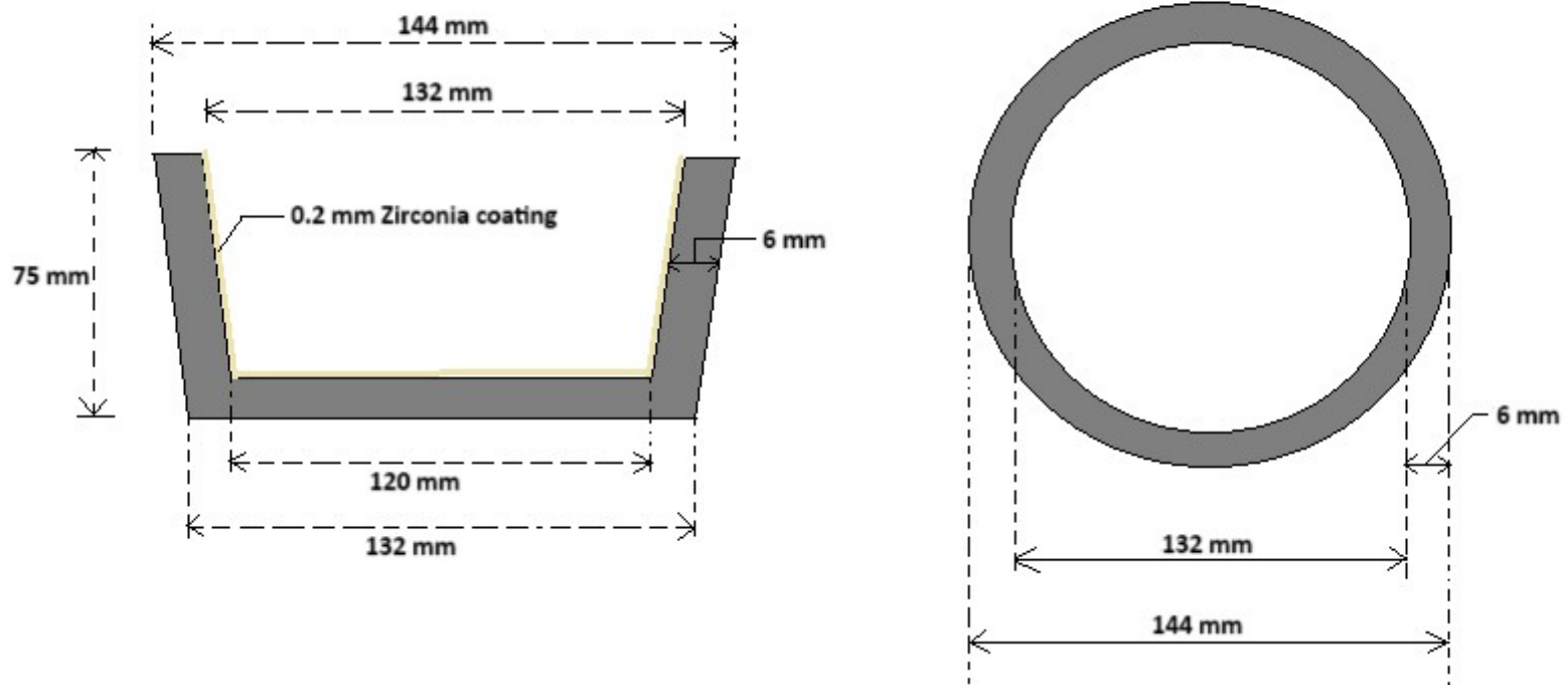
Alumina Crucible with 0.2 mm Zirconia Coating (Inside only)
