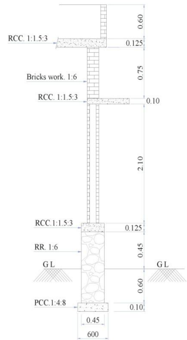
FOUNDATION DETAILS
