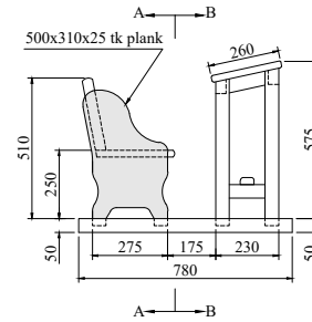
BENCH WITH DESK
