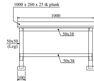
VIEW-BB
