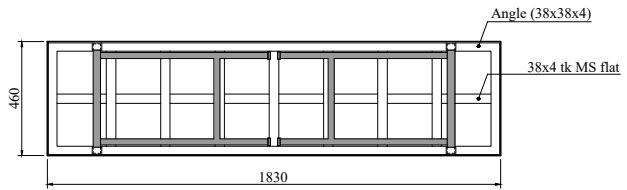
BOTTOM VIEW
