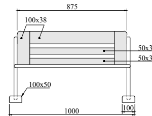
VIEW-AA
