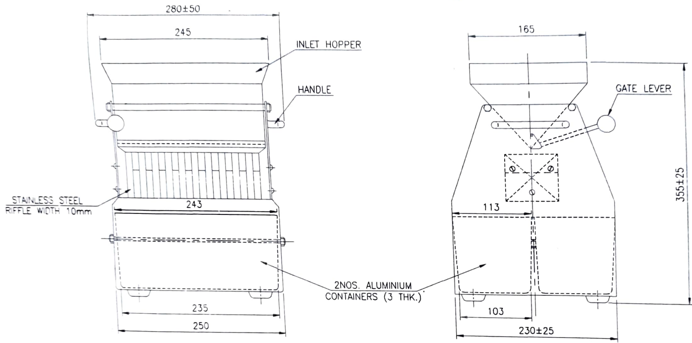
MINERAL SAMPLE SPLITTER
